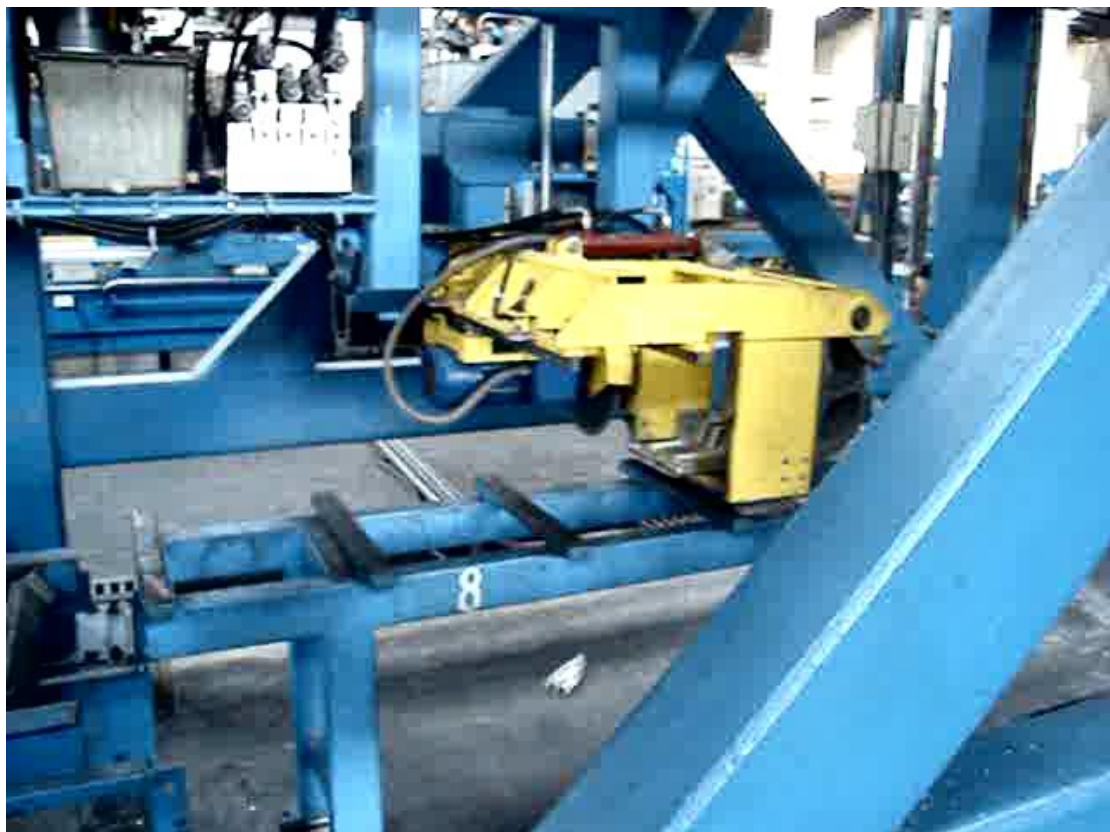
(6) 牽引機夾頭和飛鋸。Jaws and Flying Saw of Puller.
